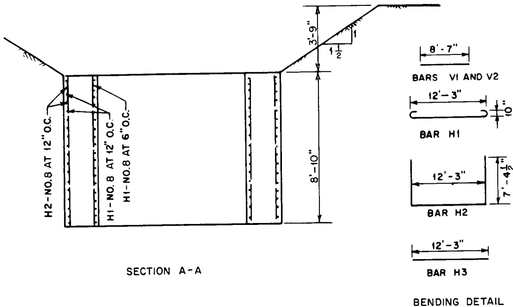
Fig. 1—Construction drawings for test structure.
